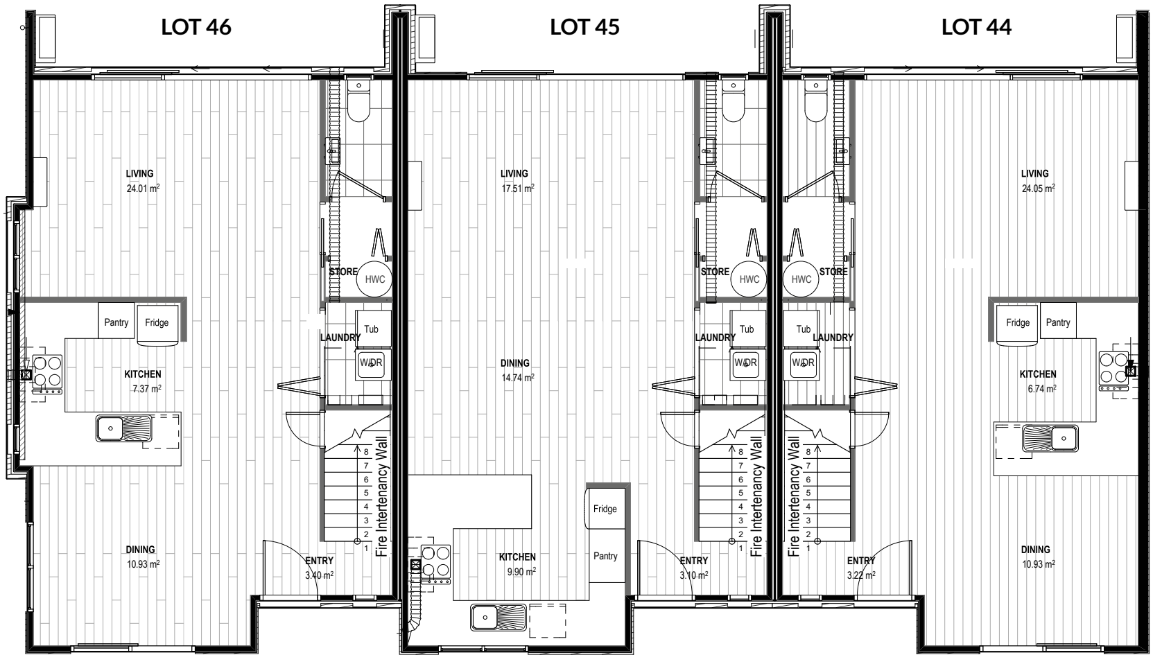
GROUND FLOOR
