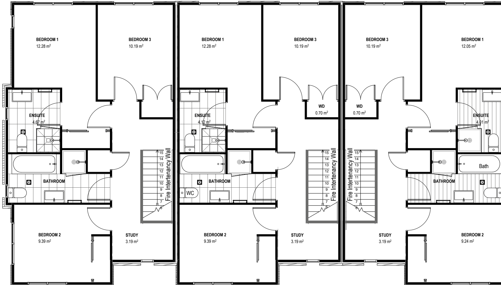
FIRST FLOOR
